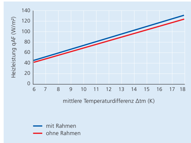
Heizleistung TBM-System mit/ohne Rahmen
