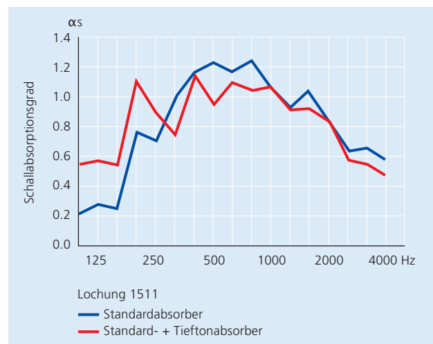
Schallabsorptionsgrad
